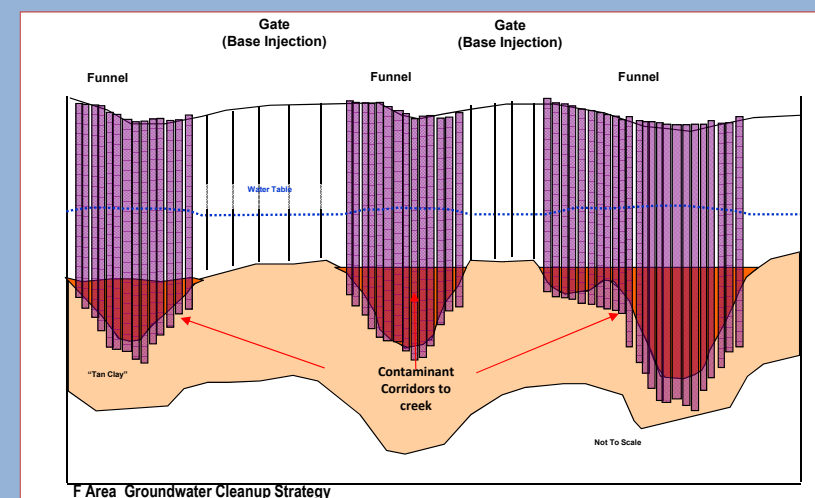
Subsurface Barriers form Funnel and Gate System in F Area
