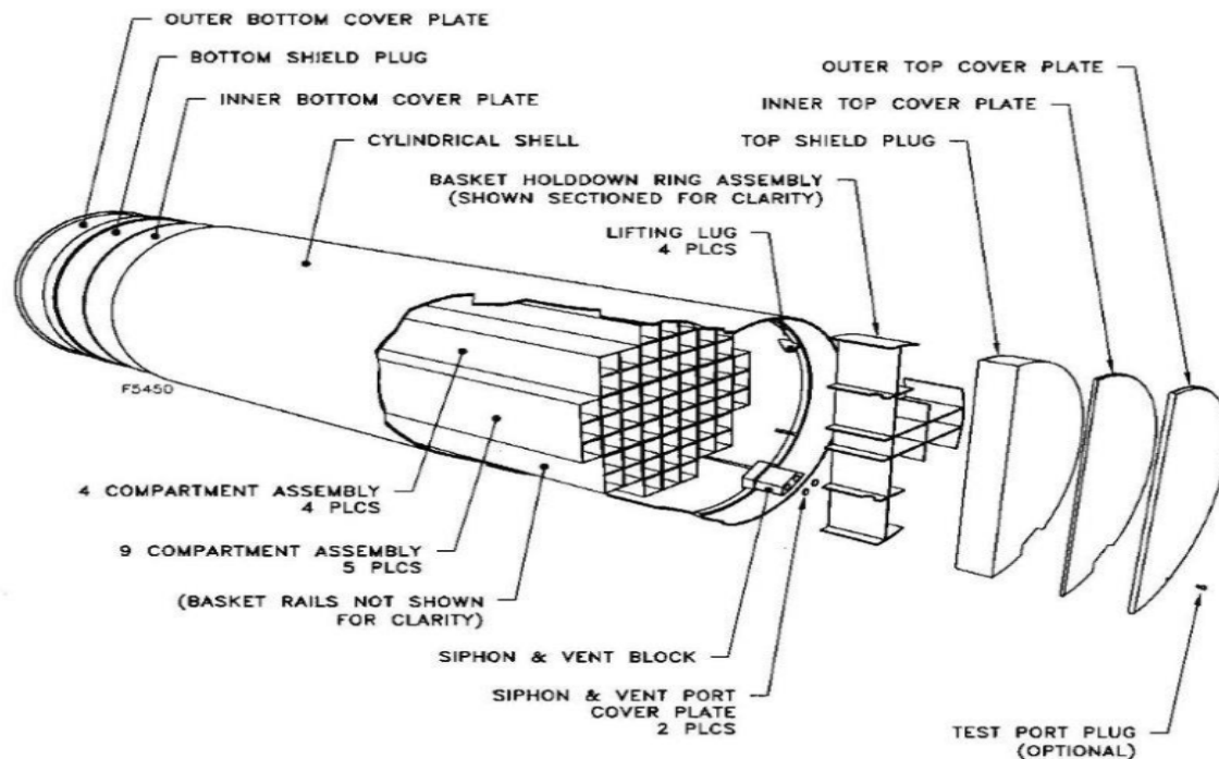
Figure 4. 61BTH Cross Section
