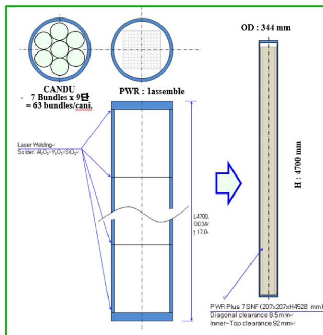
Fig. 4. DBD disposal container concept
