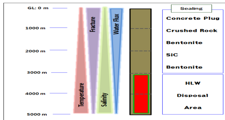
Figure 2. Deep borehole disposal environment.
