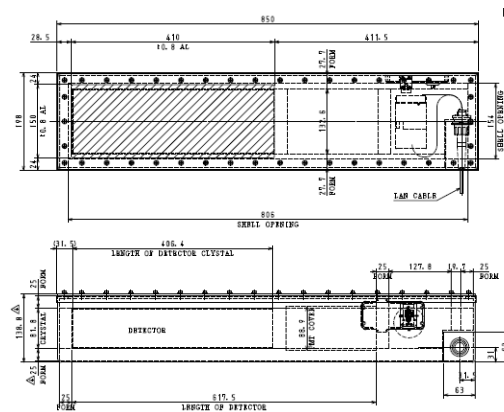
Fig.2. The drawing of detector box
