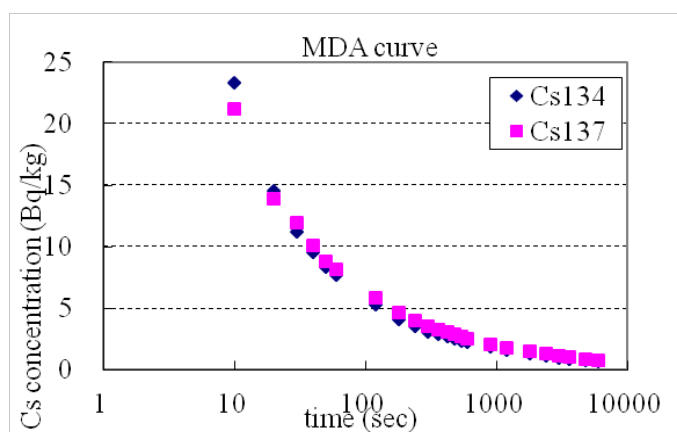
Fig. 6. MDA curve of FRAS
