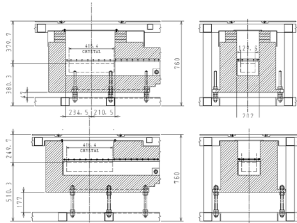
Fig.1. The drawing of shield
