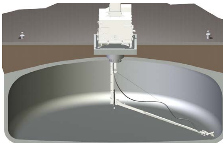
Fig. 3. Schematic of the Mobile Arm Retrieval System (MARS)
