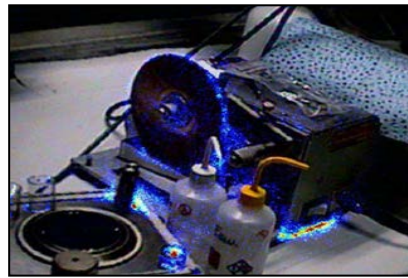
Fig. 2. Alpha camera.
