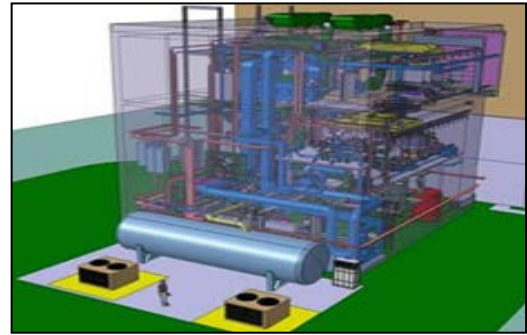
Fig .13. Sodium treatment facility
