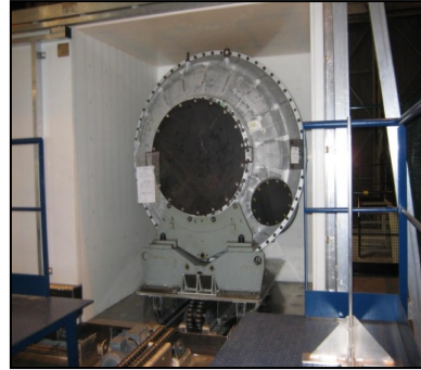
Fig .8 . Passive neutronic measurement of Uranium
