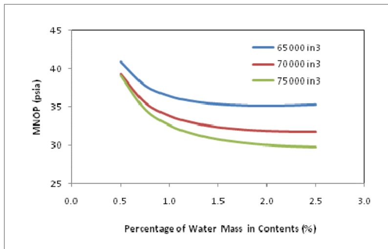
Fig. 7. MNOP vs. percentage of water mass to limit hydrogen generation to less than 5% in volume ( M_{CC} = 5,000 lb, \rho_{CC} = 0.080 lb/in 3 , G_w = 1.6 molecules/100eV).
