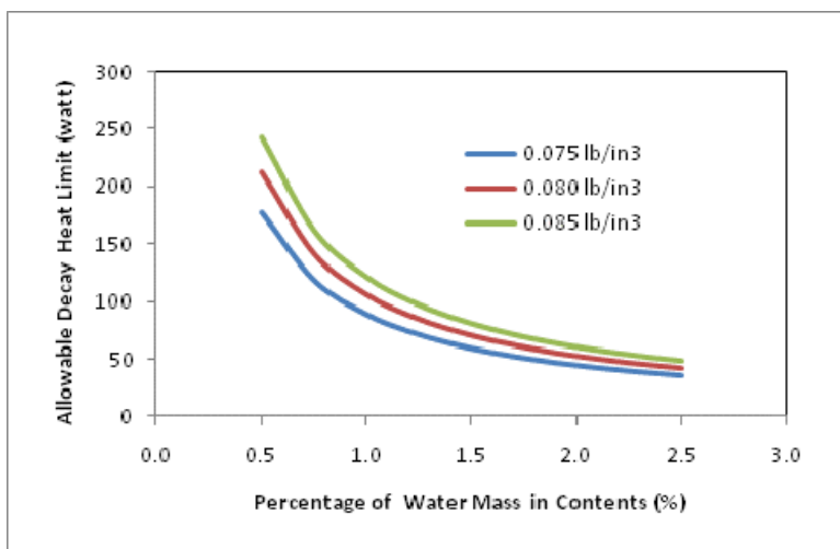
Fig. 2. Decay heat limit vs. percentage of water mass in contents to limit hydrogen generation to less than 5% in volume ( M_{CC} = 5,000 \text{ lb} , V_{CAVITY} = 70,000 \text{ in}^3 , and G_w = 1.6 \text{ molecules/100eV} ).
