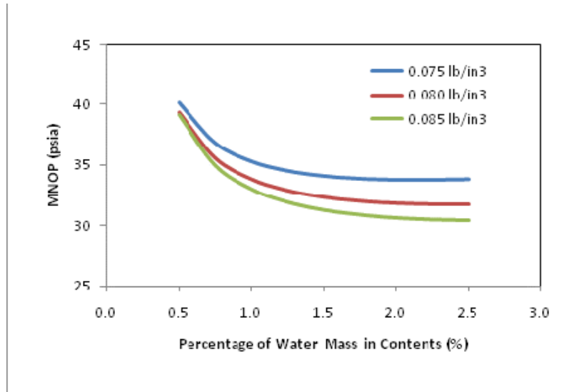
Fig. 6. MNOP vs. percentage of water mass in contents to limit hydrogen generation to less than 5% in volume ( M_{CC} = 5,000 lb, V_{CAVITY} = 70,000 in 3 , G_w = 1.6 molecules/100eV).
