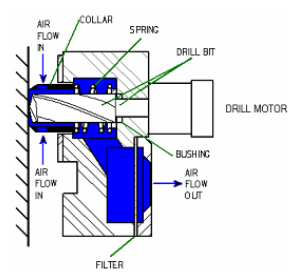
Sampler head components
