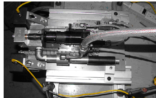
Assembled sampler head
