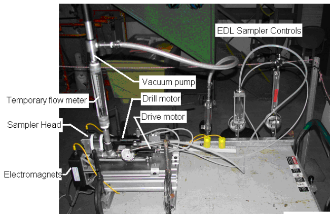
Sampler components
