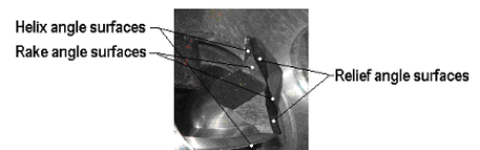
Drill bit nomenclature
