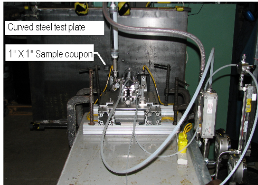
Sampler test setup
