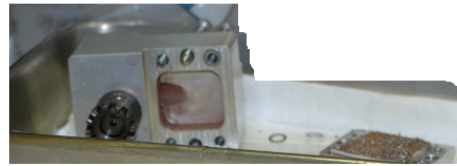
Disassembled sampler head
