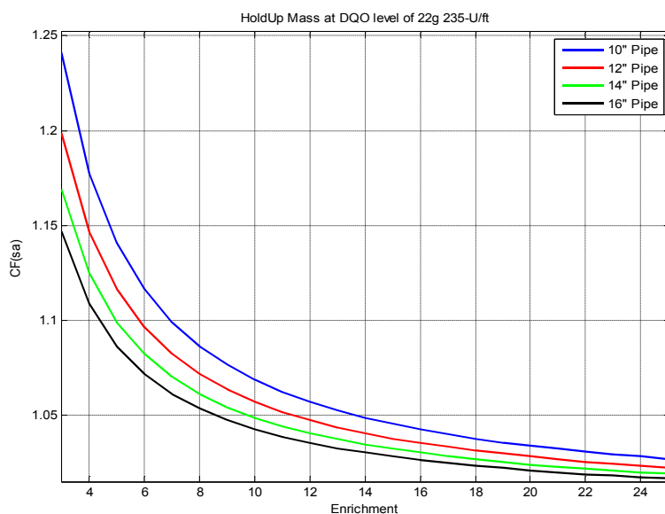
Fig. 3. Correction factor for self-attenuation as a function of enrichment (%): 22g U-235/ft.
