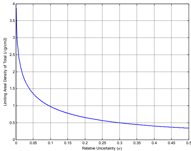
Fig. 1. Limiting corrected areal density of total uranium (Eq. 24, k=3).
