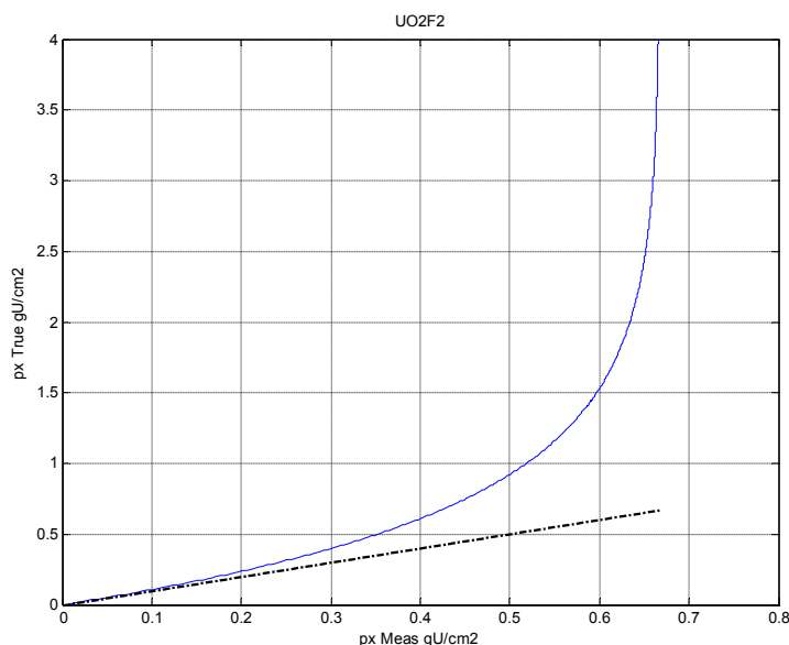
Fig. 2. Measured areal density as a function of the true (corrected) areal density of total uranium.
